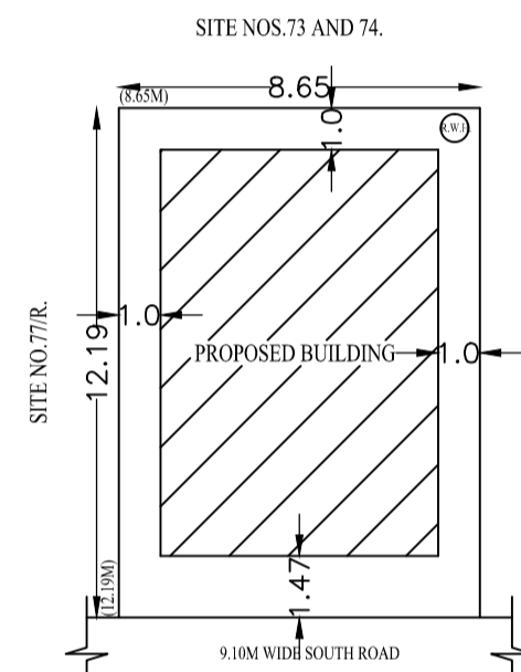
SITE PLAN
