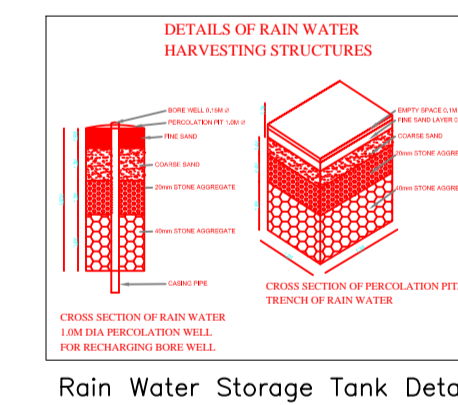
Rain Water Storage Tank Detail
